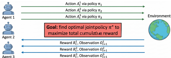
Figure 2: A Collaborative Multi-agent Reinforcement Learning-Based Framework (CREW).
